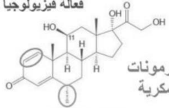
Methylprednisolone
