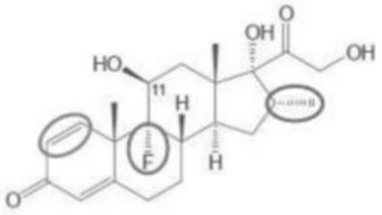
Dexamethasone
